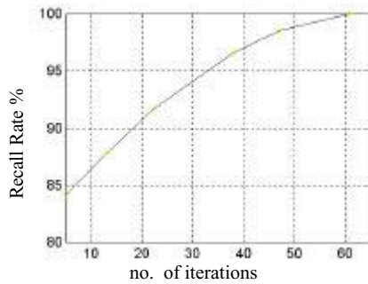
Figure 9: Diagram of the recall rate vs the no. of iterations for the recovering of image 18
