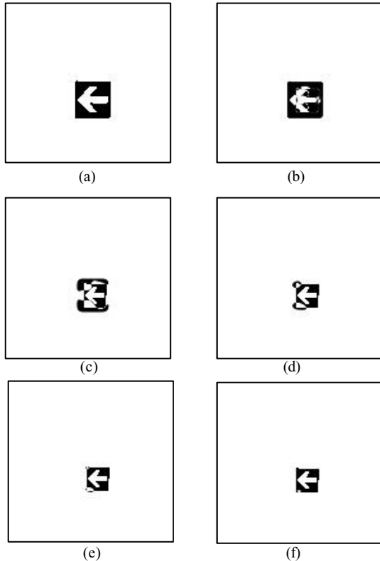
Figure 6: Recovery evolution of the designed DTCNN: (a) submitted 9-th image of the sequence; (b) output at step 1; (c) output at step 10; (d) output at step 21; (e) output at step 26; (f) final output at step 30.
