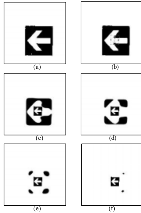
Figure 7: Recovery evolution of the designed DTCNN: (a) submitted 18-th image of the sequence; (b) output at step 1; (c) output at step 15; (d) output at step 30; (e) output at step 45; (f) final output at step 61.
