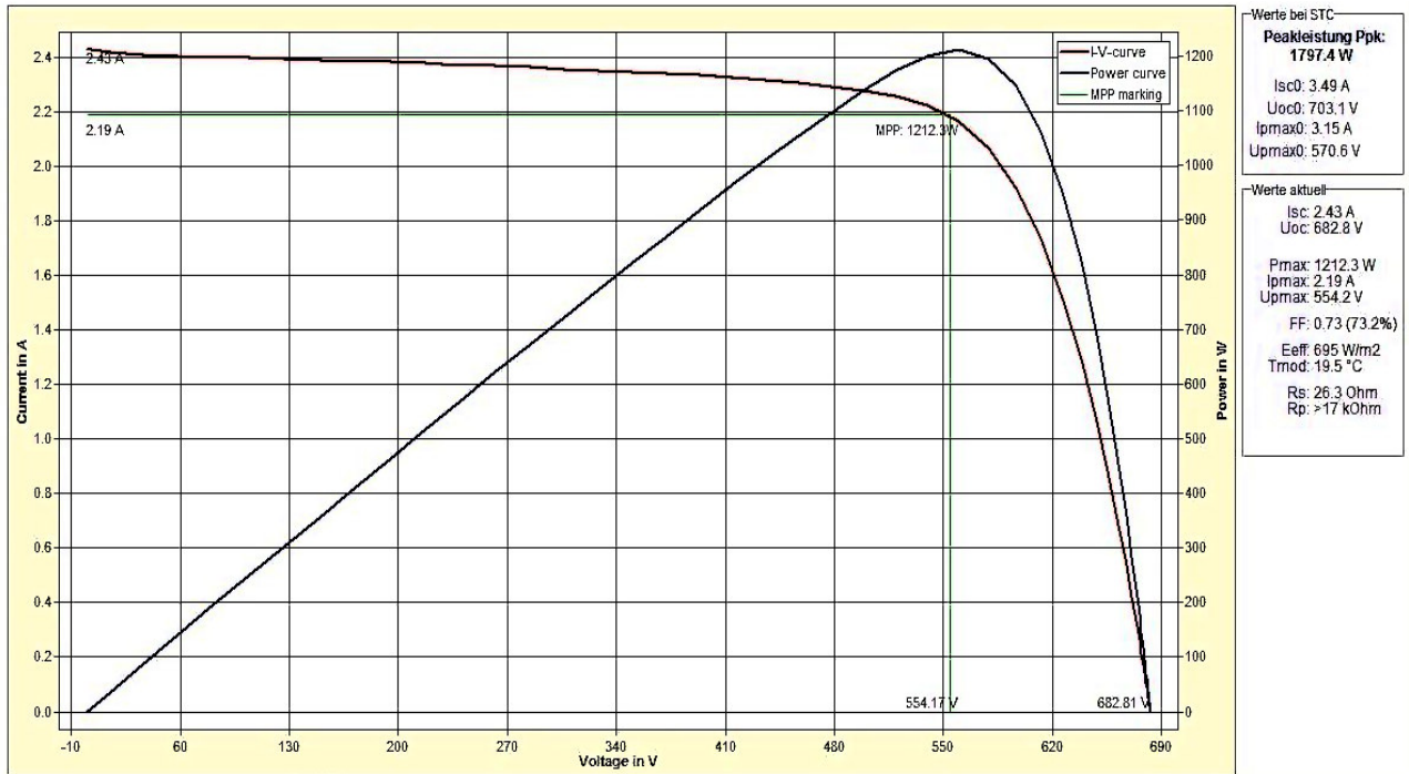
FIGURE 7: EXPERIMENTAL IV AND PV CURVES
