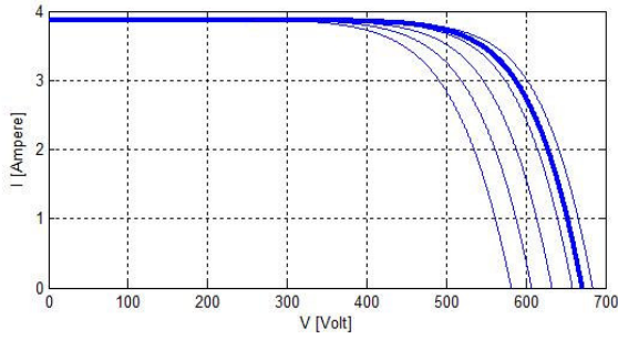
FIGURE 5: PV MODEL 2 – SERIES ARRAY SIMULATION CURVES AT VARIABLE TEMPERATURE (a) AND IRRADIANCE (b)
