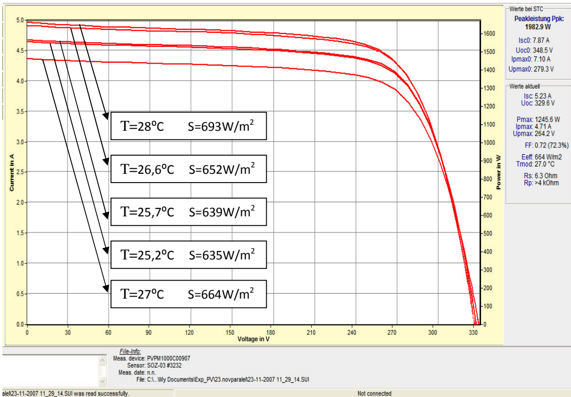
FIGURE 8: TEMPERATURE AND IRRADIANCE VARIATION CURVES (EXPERIMENTAL RESULTS)
