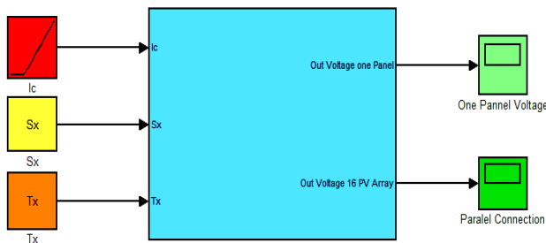
FIGURE 2: PV MODEL – SIMULATION SYSTEM BLOCK
