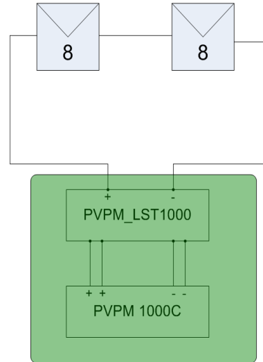
FIGURE 6: EXPERIMENTAL ARRANGEMENT
