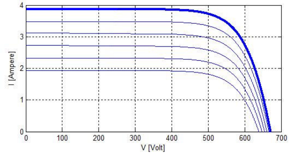
FIGURE 5: PV MODEL 2 – SERIES ARRAY SIMULATION CURVES AT VARIABLE TEMPERATURE (a) AND IRRADIANCE (b)
