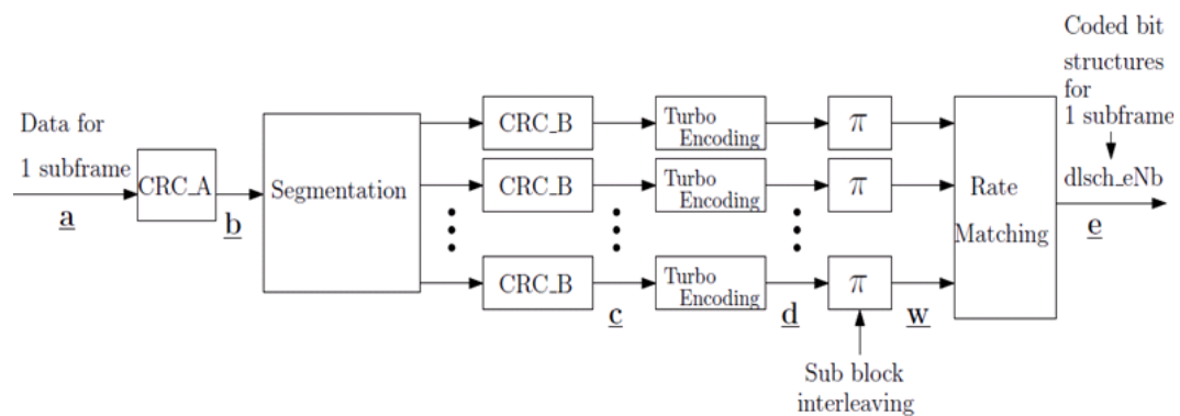
FIGURE 2.8: Channel Coding
