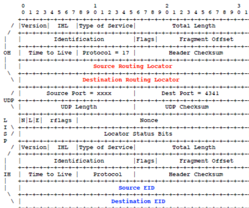
Figure 4.1: LISP Header Format
