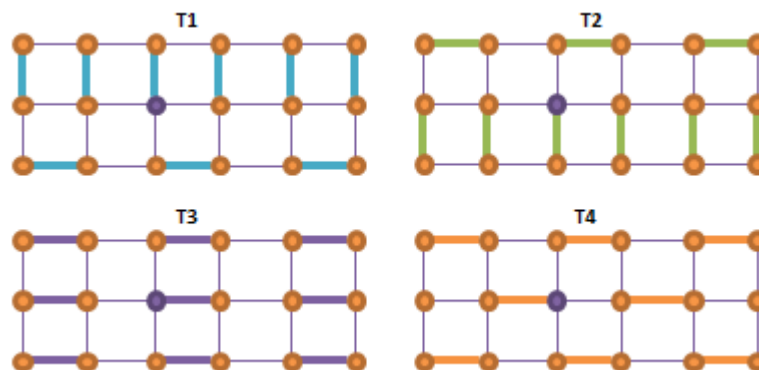
Figure 13: Example activity set (T) calculation for a “chocolate bar” topology. The purple node is the gateway node. The colored links represent the direction of the shared resources system at a given time.
