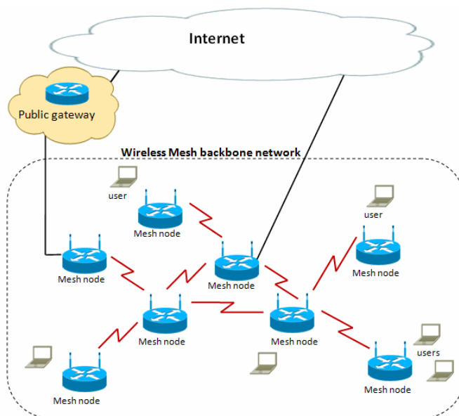
Figure 10: Reference architecture for a wireless mesh network. [85]
