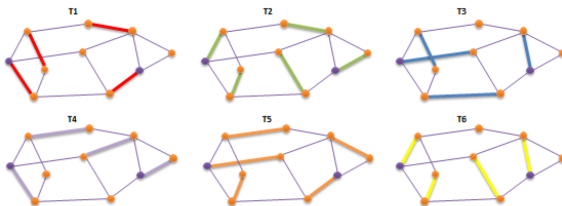
Figure 20: Calculated spanning trees for the test topology.
