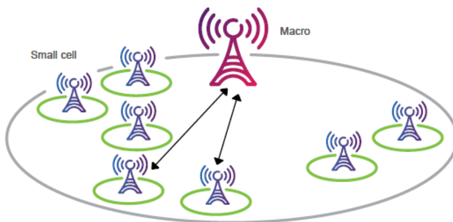
Figure 8: Heterogeneous network. [64]
