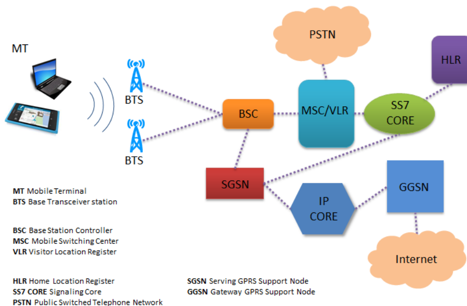
Figure 5: The structure of a GSM network enhanced with GPRS elements.
