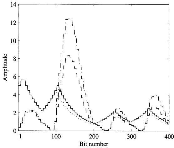
Fig. 3. A plot of the received power level estimates using the predictive (dashed) and the reference (dash-dot) controllers, along with the transmitter power level setting with the predictive (dotted) and the reference (solid) power controller. Speed of the observed mobile is 30 km/h and the total control loop delay is 127 chip durations.
