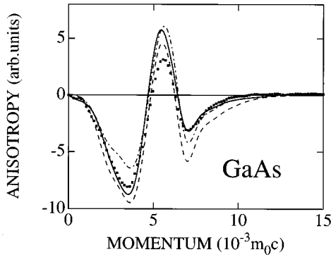
FIG. 6. Anisotropy of the 2D-ACAR spectra for the perfect bulk GaAs lattice. The momentum distributions are integrated in the [110] direction and normalized to the same value at zero momentum. The anisotropies are calculated as the differences between the distributions along the [110] and [001] directions. The solid, dashed, and dash-dotted lines are the results in the present state-dependent enhancement scheme, in the GGA of Eq. (6), and in the IPM, respectively. The experimental points are given by dots.
