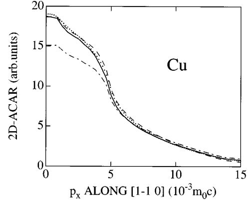
FIG. 3. 2D-ACAR spectra for Cu. The momentum densities are integrated in the [111] direction, and normalized to the same volume. Cuts along the [110] direction are given. The solid, dashed, and dash-dotted lines give the results in the present state-dependent enhancement scheme, in the GGA of Eq. (6), and in the IPM, respectively. The experimental points are shown by dots.
