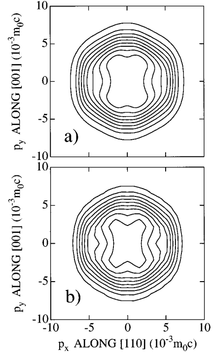
FIG. 5. Experimental (a) and theoretical (b) 2D-ACAR spectra for the perfect bulk GaAs lattice. The momentum distributions are integrated in the [110] direction and normalized to the same value at zero momentum. The contour spacing is one tenth of the maximum value.
