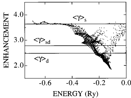
FIG. 2. Enhancement factors for the conduction band states in Cu. The horizontal lines give the values obtained using the atomic superposition method for the 4s ( \langle\gamma_s\rangle ) and 3d ( \langle\gamma_d\rangle ) electrons as well as their weighted average ( \langle\gamma_{sd}\rangle ). The energy zero coincides with the Fermi level.
