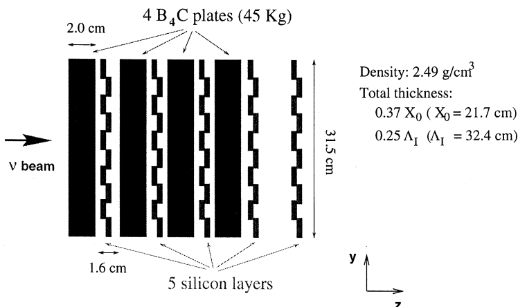
Fig. 2. Schematic of the side view of the silicon target.
