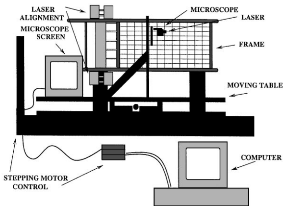
Fig. 14. Systems used for surveying the layers of NOMAD-STAR.
