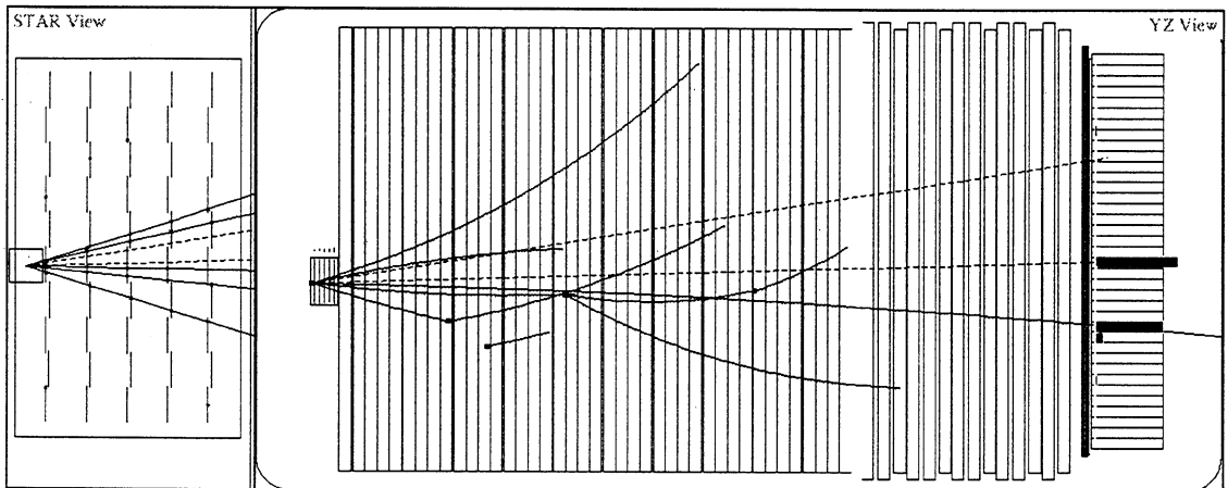
Fig. 4. Reconstructed \nu_\mu charged current interaction inside the B_4C -silicon target (expanded view of the target is shown on the left).
