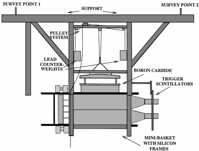
Fig. 16. Support system for NOMAD-STAR with mini-basket and silicon layers.
