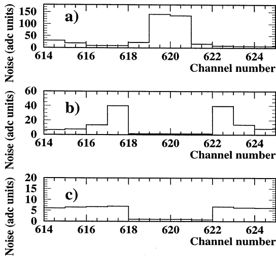
Fig. 8. Noise for all channels of a typical ladder with (a) very noisy strips, (b) noisy strips removed and (c) noisy strips grounded.
