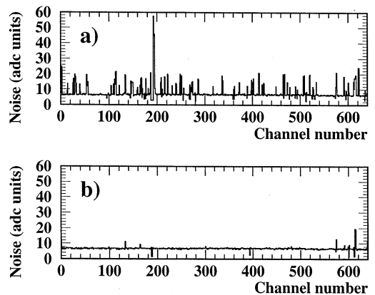
Fig. 12. Noise for all channels of a typical ladder with: (a) several short-circuited strips and (b) short-circuited wires separated.
