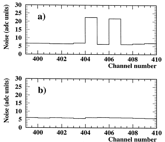
Fig. 10. Noise for all channels of a typical ladder with (a) shorted strips, and (b) shorted wires separated.
