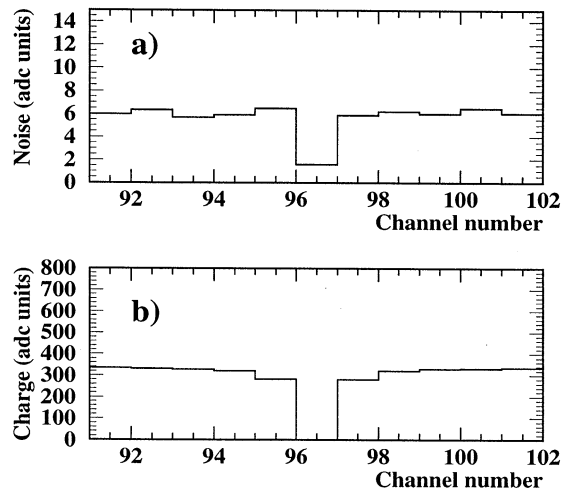
Fig. 9. (a) Noise, and (b) measured strip charges with backplane pulsing for a typical ladder with an interrupted strip.
