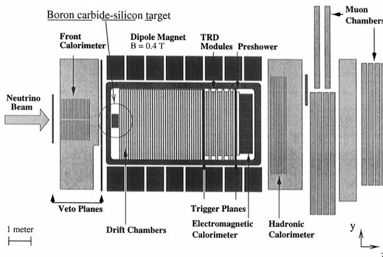
Fig. 1. The NOMAD detector with the boron carbide-silicon target (NOMAD-STAR).
