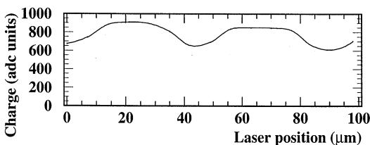
Fig. 11. Total charge collected by the strips.
