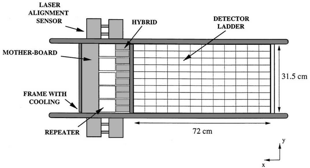
Fig. 3. Individual silicon layer with 10 ladders and 12 detectors per ladder.
