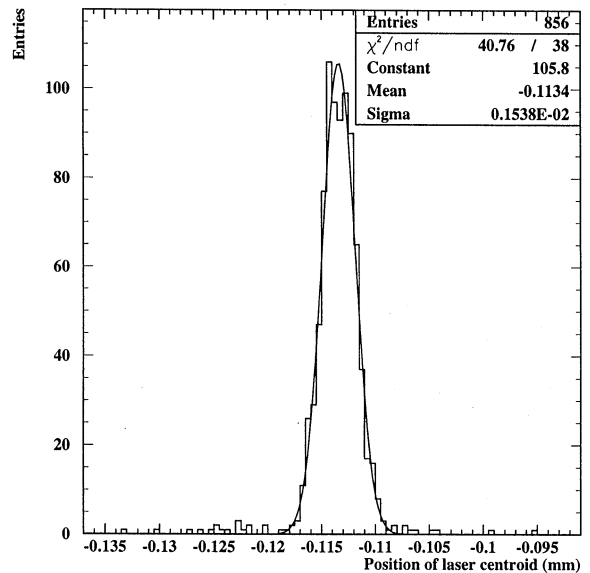
Fig. 17. Position resolution for a typical sensor used in laser alignment system. The width of the distribution corresponds to the resolution of the sensor ( 1.5\ \mu\text{m} ).
