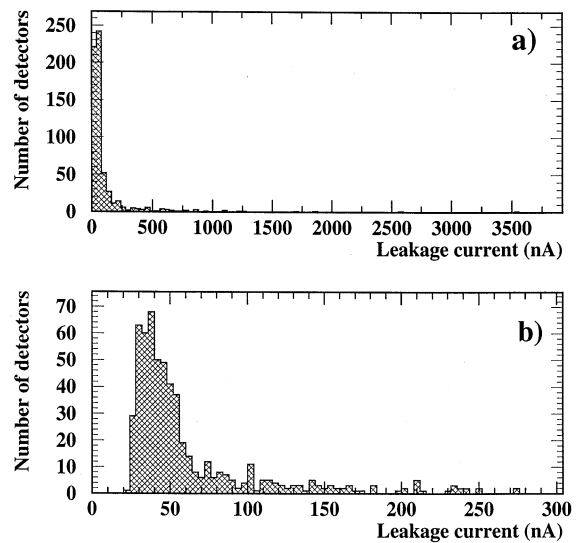
Fig. 5. Leakage current distributions for: (a) all detectors, (b) only detectors with leakage current smaller than 300 nA.
