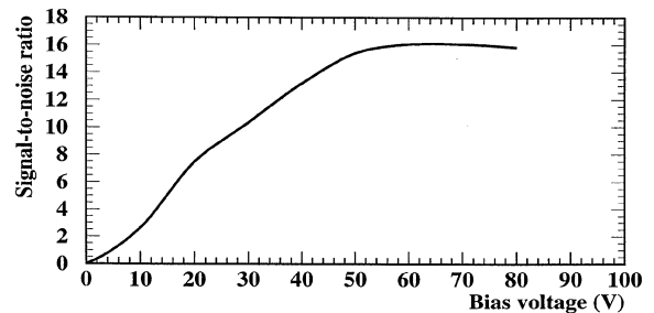
Fig. 7. Signal-to-noise ratio versus bias voltage for a typical ladder.
