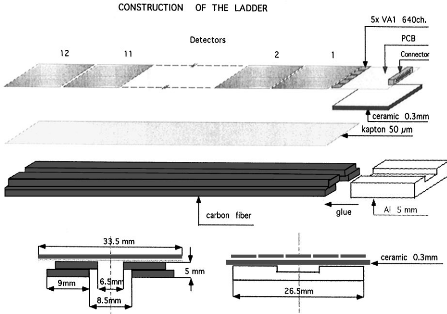
Fig. 6. Schematical drawing of a ladder.
