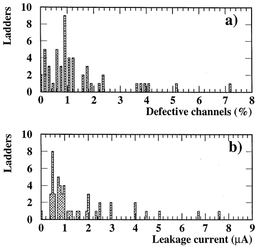
Fig. 13. (a) Percentage of defective channels for all ladders, and (b) leakage current for all ladders.
