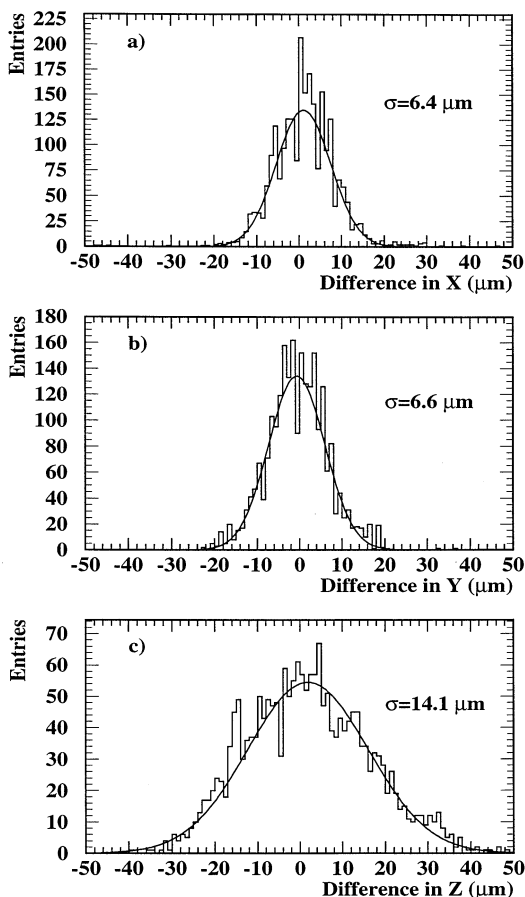
Fig. 15. Resolution of the surveying system. Systematic differences in the measurements of the coordinates (a) X , (b) Y and (c) Z .
