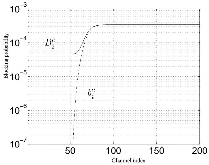
Figure 6 Channel B_i^c and call blocking probabilities b_i^c for each channel ( B_i^c solid line, b_i^c dashed line).
