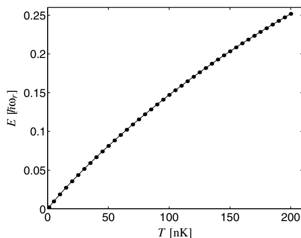
FIG. 2. Energy of the lowest excitation, the LCLS, at temperatures T = 1 –200 nK ( T_c \approx 1 \mu\text{K} ). The finite positive value of the lowest excitation frequency implies the vortex to be locally energetically stable.
