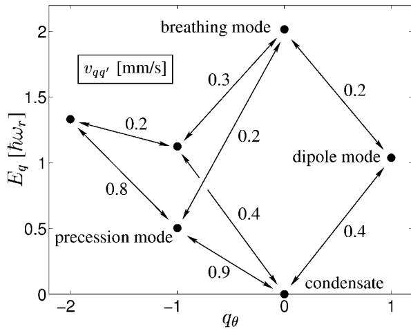
FIG. 1. Adiabaticity velocities determined by decay rates between the lowest vortex state excitations (dots) with q_z = 0 . The data correspond to the PA and system temperature T \approx 0.8T_{\text{BEC}} . The arrows denote the decay channels of the modes to each other, and the numbers the corresponding adiabaticity velocities v_{qq'} [mm/s] [see Eq. (21)]. Note especially the low adiabaticity velocity given by the transitions between the precession and breathing modes—transitions from the precession mode are crucial in determining the deformation of the core structure of a moving vortex. Furthermore, due to weaker mutual couplings, the adiabaticity velocities given by transitions between states with higher energy or q_z \neq 0 were, in general, found to be larger. The degree of adiabaticity of a moving vortex is thus essentially determined by the lowest collective modes.
