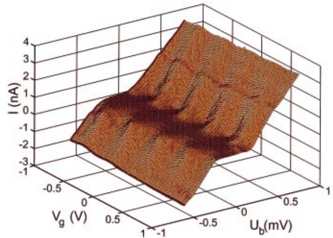
FIG. 3. (Color) Current of the nanotube SET as a function of gate voltage V_g and bias voltage U_b . The Coulomb blockade is clearly seen in the rhombic regions in the center.
