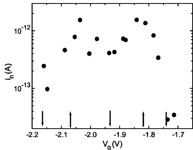
FIG. 4. Current noise ( i_n ) measured over one modulation period of the gate voltage in the regime of the Coulomb blockade. The bias voltage ( U_b ) was 0.4 meV. Arrows indicate points of maximum (up arrows) and minimum (down arrows) gain.
