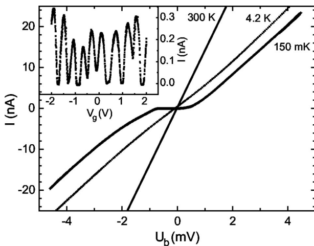
FIG. 2. Current-voltage characteristics of the lower tube at different temperatures. Inset: gate modulation of the current at T = 150 mK and U_b = 0.4 mV.
