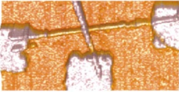
FIG. 1. (Color) AFM image of the fabricated multiwalled nanotube device. The lower tube has gold contacts at both ends, while the upper tube has only one end contacted (at the bottom of the image).
