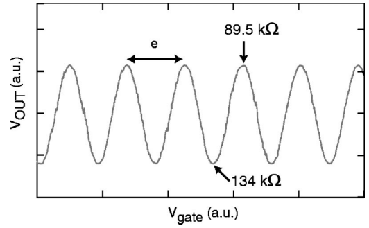
FIG. 10. Measured transfer function, i.e., output voltage from detection vs gate voltage. One period corresponds to a change of charge by e on the island. The minimum and maximum values of V_{\text{OUT}} correspond to R_{\text{SET}} = 134 and 89.5 k \Omega , respectively.
