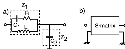
FIG. 17. (a) Lumped-element representation of LC matching circuit. Impedances Z_1 and Z_2 represent the total impedance of the corresponding dashed boxes. (b) Equivalent S -matrix representation.
