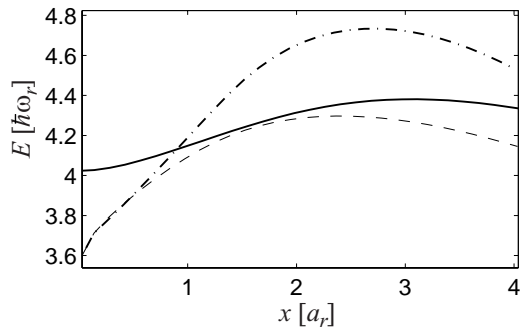
FIG. 2: Energy of the vortex dipole (dashed line), tripole (solid line) and quadrupole (dash-dotted line) as functions of the distances d_2 , d_3 and d_4 , respectively. The strength of the interactions is \tilde{g} = 160 for all the configurations.
