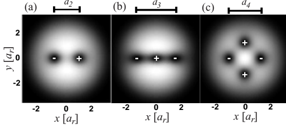
FIG. 1: Density profiles of a stationary vortex dipole (a), tripole (b) and quadrupole (c). The separations of the outermost vortices are marked by d_2 , d_3 and d_4 for the dipole, tripole and quadrupole, respectively. The plus signs in the vortex core denote vortices and minus signs antivortices. The strength of the interactions \tilde{g} is 170 for the vortex dipole and 160 for the tripole and quadrupole.
