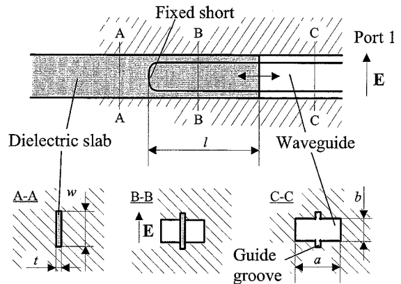
Fig. 1. Structure of the new tunable backshort.
