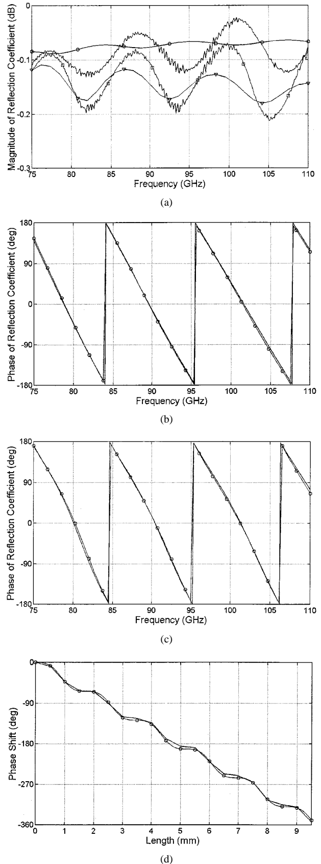
Fig. 2. Reflection coefficient S_{11} . (a) |S_{11}| for l = 0 (measured: solid line; simulated: line with circles) and for l = 9.5 mm (measured: line with squares; simulated: line with triangles); (b) measured and simulated (line with circles) phase for l = 0 ; (c) measured and simulated (line with circles) phase for l = 9.5 mm and (d) Measured and simulated (line with circles) \Delta\phi as a function of l at 92.5 GHz.
