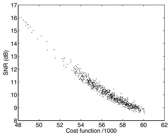
Fig. 3. Signal-to-noise ratio of the optimal linear reconstruction of the true sources from the estimated source subspace as a function of the cost function value attained in different stages of different simulations, some of which were run for up to 50000 iterations
