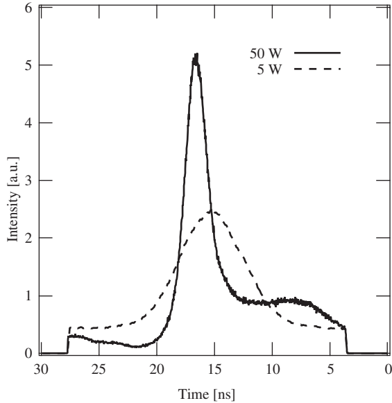
Fig. 2. Increasing the chopping power from 5 W to 50 W improves pulse width but changes the pulse shape due to scattering and secondary electron effects.
