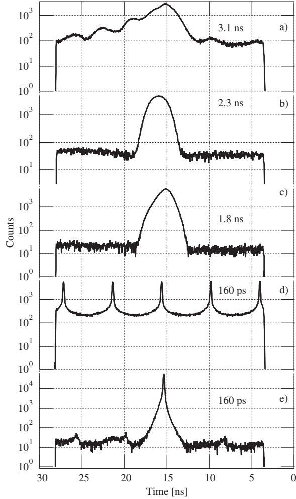
Fig. 3. The spectra measured from bunchers and the chopper and their combinations show that a time resolution of 160 ps, is obtainable with the sawtooth chopper. a) prebuncher, b) chopper, c) prebuncher and chopper, d) buncher and e) all together. The FWHM for each component and combinations of them is given in the figure.
