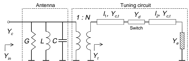
Fig. 1. Circuit model for frequency-tunable resonant antenna with series switch. Load admittance Y_e represents the open ( Y_e = 0 ) or shorted ( Y_e = \infty ) end of line 2.
