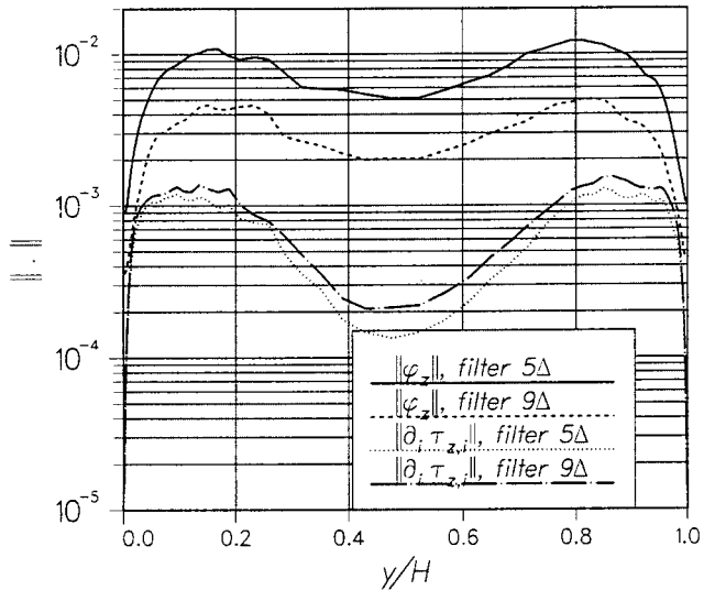
Figure 51. The L_2 -norm of the estimated discretization error \|\phi_z\| and the subgrid term \|\partial\tau_{z,x_i}/\partial x_i\| in the spanwise direction.
