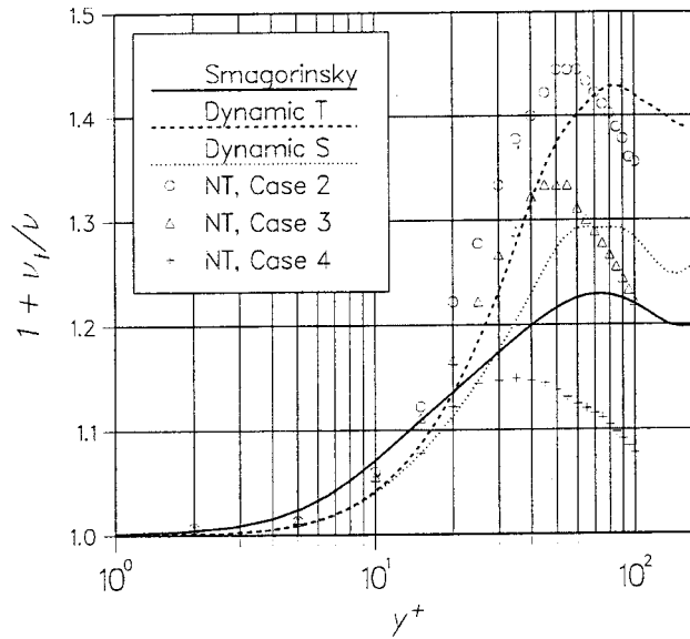
Figure 28. The eddy viscosity produced by the subgrid-scale models with the medium grid. The reference solution is from Najjar and Tafti [9].
