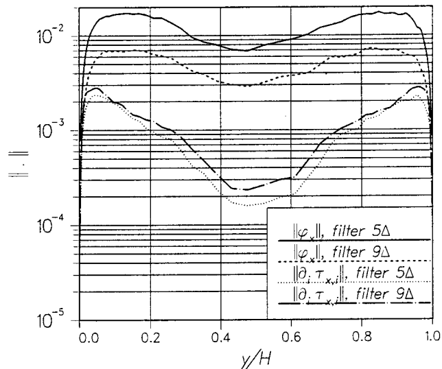
Figure 49. The L_2 -norm of the estimated discretization error \|\varphi_x\| and the subgrid term \|\partial \tau_{x,i} / \partial x_i\| in the streamwise direction.
