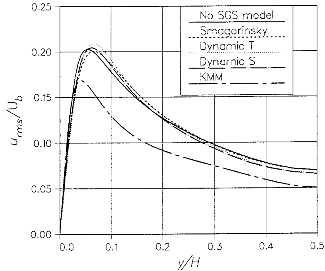
Figure 14. The rms fluctuations of u : \sqrt{u'u'}/U_b . The results are from the coarse-grid simulations.
