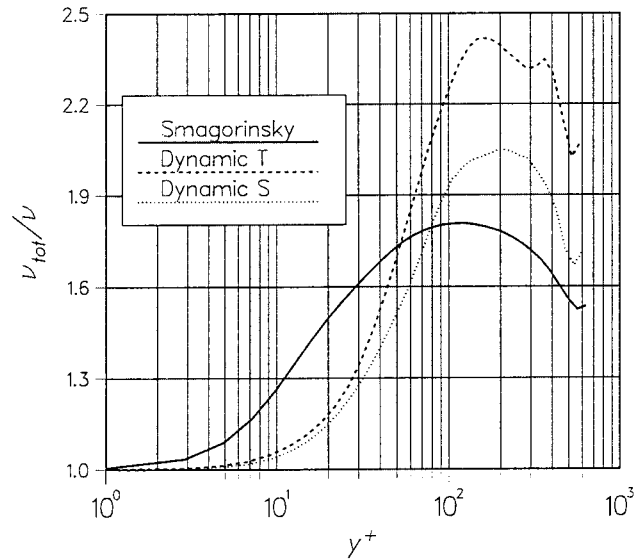
Figure 48. The scaled subgrid scale viscosity (v + v_t)/v at Re_b = 12500 .
