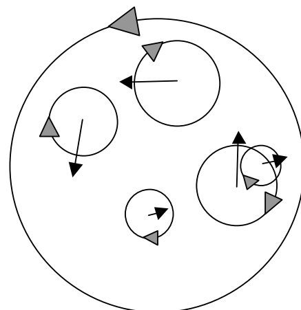
Figure 5. The forces in the galaxy.
