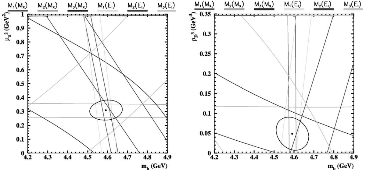
Fig. 1. The projection of the constraints of the six measured moments on the m_b(1 \text{ GeV})-\mu_\pi^2(1 \text{ GeV}) (left) and m_b(1 \text{ GeV})-\rho_D^3 (right) planes. The bands correspond to the total measurement accuracy and are given by keeping all the other parameters at their central values. The ellipses represent the 1\sigma contours.
