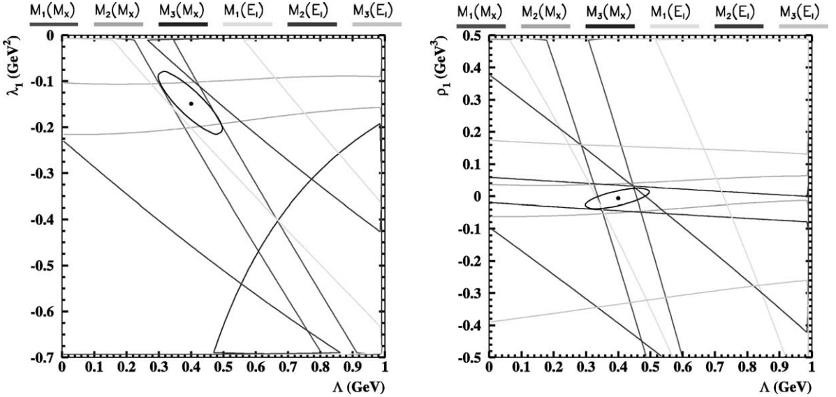
Fig. 2. The projection of the constraints of the six measured moments on the \bar{\Lambda}-\lambda_1 (left) and \bar{\Lambda}-\rho_1 (right) planes. The bands correspond to the total measurement accuracy and are given by keeping all the other parameters at their central values. The ellipses represent the 1\sigma contours.
