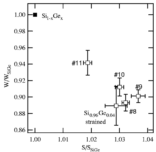
FIG. 5. The S and W parameters in the irradiated samples relative to the as-grown ones show that in all the n -type samples the irradiation induced defects have a similar structure.
