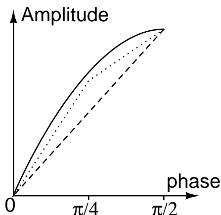
Figure 3.6 Trigonometric approximations: sine-phase difference (dashed) and double trigonometric (dotted)
