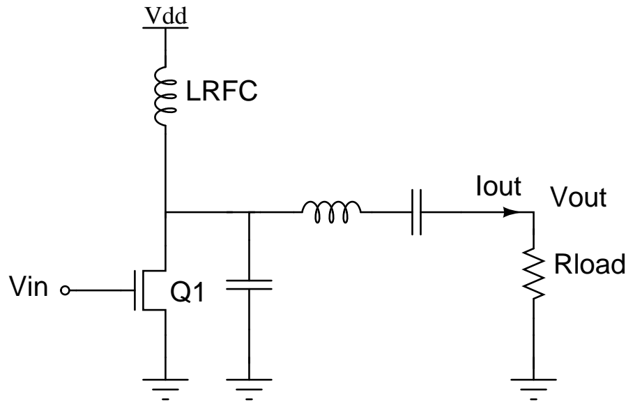
Figure 5.1 Class-E amplifier
