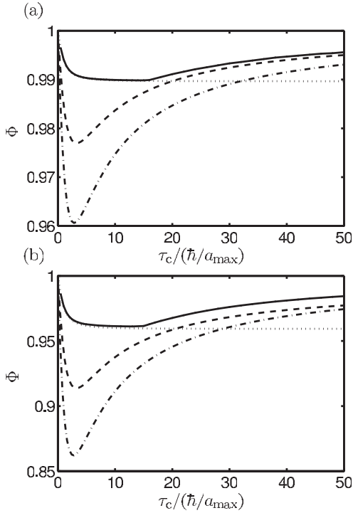
FIG. 1. Fidelities for the NOT gate as functions of the correlation time \tau_c for a \pi -pulse (dotted line), CORPSE (dashed-dotted line), short CORPSE (dashed line), and gradient optimization (solid line). The RTN strength \Delta is set to (a) 0.125a_{\max} and (b) 0.25a_{\max} . The gate fidelity for a gate U is defined as \langle \text{Tr}[U\rho_0 U^\dagger \rho] \rangle , where the average is calculated over all pure initial states \rho_0 , see Ref. [11].
