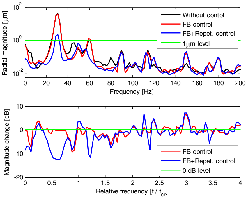
Figure 49. The rotor midpoint responses with repetitive control when running at 30 rps.
