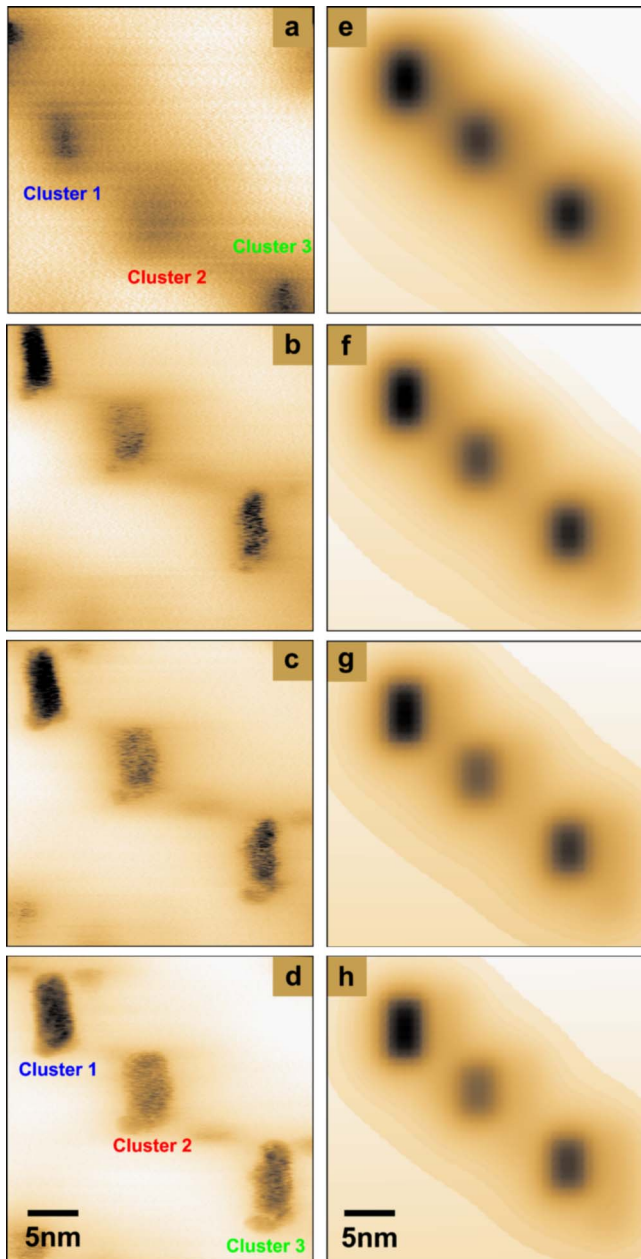
FIG. 5. (Color online) Experimental images (a)–(d) of three Pd clusters imaged in the region ( 30 \times 30 \text{ nm}^2 ) of the dotted square in Fig. 4(a) and corresponding calculated images (e)–(h). The preset value of \Delta f was decreased during the measurements from image to image [ -7.6 (a), -12.6 (b), -15.6 (c), and -18.7 Hz (d)]. Scan speed: v_{\text{scan}} = 10 Hz. The theoretical images (e)–(h) were calculated at the following tip-cluster distances: 1.2 (e), 0.7 (f), 0.5 (g), and 0.4 nm (h).
