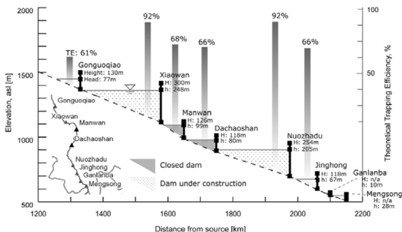
Fig. 10. Profile of the Lancang Cascade of dams plotted with the location, height, head, and average theoretical trapping efficiency of each reservoir (source: Dore and Yu, 2004; McCormack, 2001; Plinston and He, 1999).
