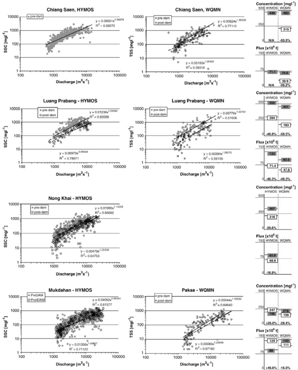
Fig. 7. The suspended sediment concentration plotted against the discharge for selected stations.
