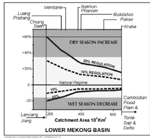
Fig. 9. Potential changes to average wet and dry season flows in the Lower Mekong channel, given 10 and 20% regulation by hydropower dams in Yunnan (Adamson, 2001). Reproduced with permission from International Water Power and Dam Construction.
