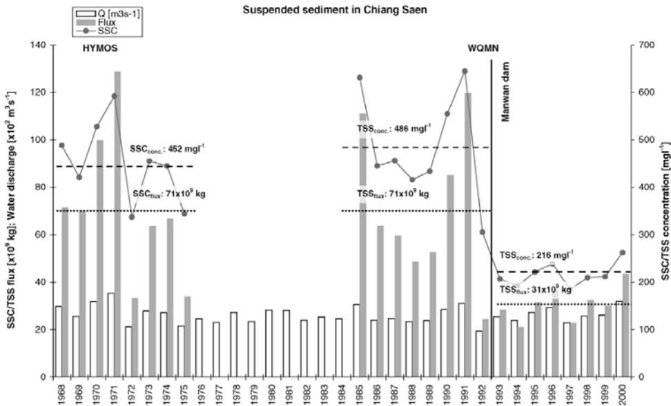
Fig. 6. Annual SSC and TSS flux ( \times 10^9 kg), SSC and TSS concentrations ( \text{mg l}^{-1} ), and discharge ( \text{m}^3 \text{s}^{-1} ) at Chiang Saen, northern Thailand. Annual average SSC and TSS concentrations and fluxes are presented for three periods (1968–1975, 1985–1992, and 1993–2000).
