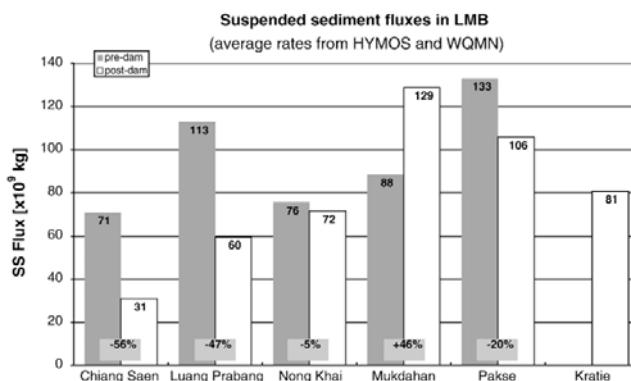
Fig. 5. Suspended sediment fluxes in the lower basin (LMB), before and after dam closure: averages from HYMOS and WQMN datasets.
