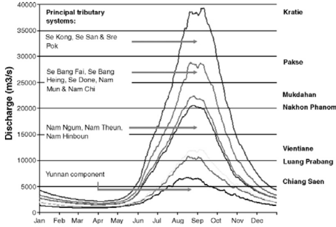
Fig. 2. Mean flows at selected sites in the Mekong mainstream, and an indication of the major tributaries and their contribution in each reach. Hydrographic data from 1960–2000 from Mekong River Commission (2004) .
