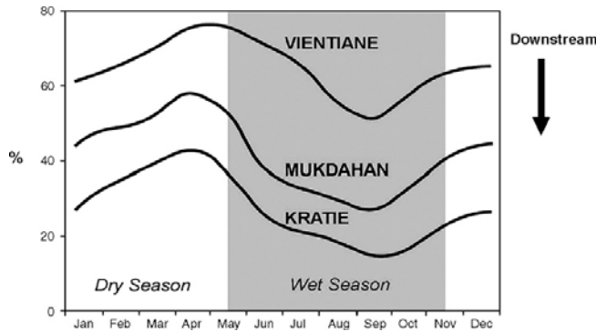
Fig. 3. Mekong River: percentage contribution of the Upper Mekong Basin to mean monthly flow at selected sites ( Adamson, 2001 ). Reproduced with permission from International Water Power and Dam Construction.
