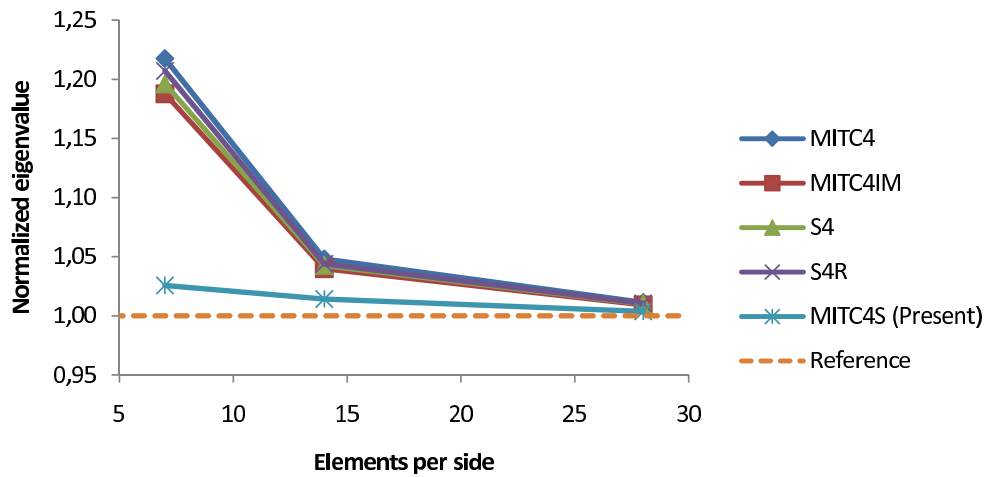
Figure 18: Convergence of the lowest eigenvalue of the hyperbolic paraboloid at R/t = 100 : uniform N \times N meshes with N = 7, 14, 28 .
