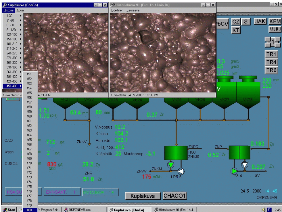
Figure 4: Graphical User Interface of the Froth Image Browser – program
