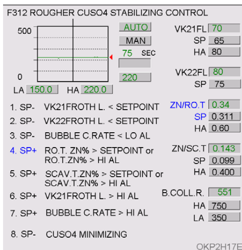
Figure 6: Copper sulphate control logic
