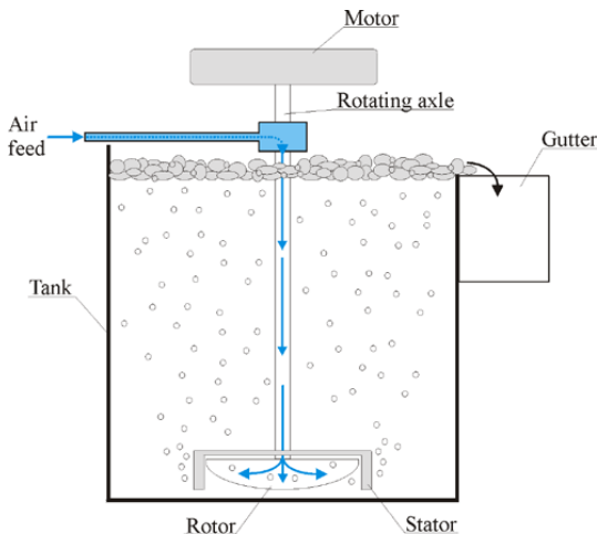
Figure 1: Main parts of a flotation cell
