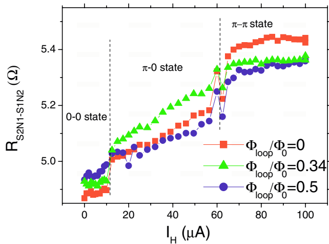
FIG. 3 (color online). Data from Fig. 2 presented as a function of I_H at different values of \Phi_{loop} . We identify the different regions with the phase states in Fig. 1(c).
