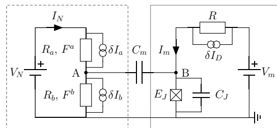
FIG. 1. Noise measurement circuit. The voltage noise at point A, driven with V_N , induces voltage noise at point B through the capacitor C_m and in this way affects JJ. JJ is in a highly resistive environment, R > R_Q = h/(4e^2) . F_n^{a,b} are the Fano factors for the n th cumulants in the noise source. The noise is read by investigating I_m(V_m) , as explained in the text.
