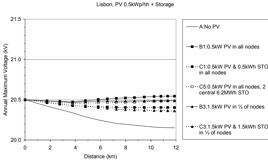
Figure 4.4: Annual maximum voltage profiles in Lisbon for cases A, B1, B3, C1, C3, and C5. The installed PV capacity totals 0.5 \text{ kW}_p / \text{hh} , and the corresponding storage capacity 0.5 \text{ kWh} / \text{hh}
