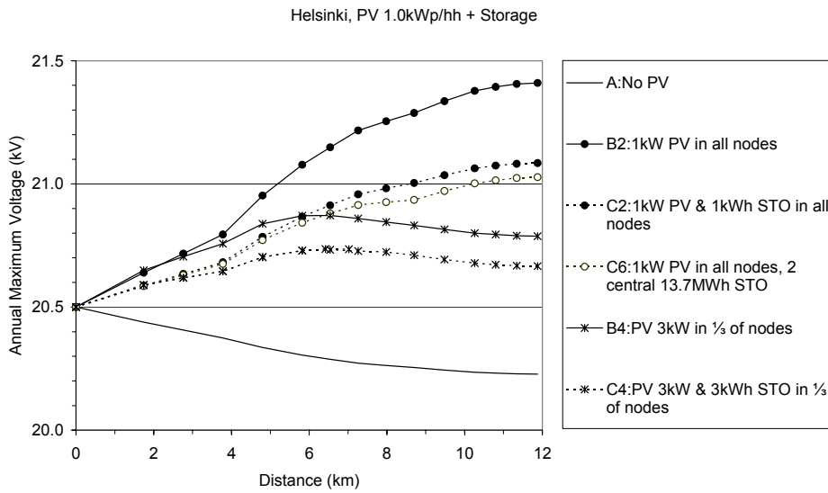
Figure 4.3: Annual maximum voltage profiles in Helsinki for cases A, B2, B4, C2, C4, and C6. The installed PV capacity totals 1.0 \text{ kW}_p / \text{hh} and the corresponding storage capacity 1.0 \text{ kWh} / \text{hh}
