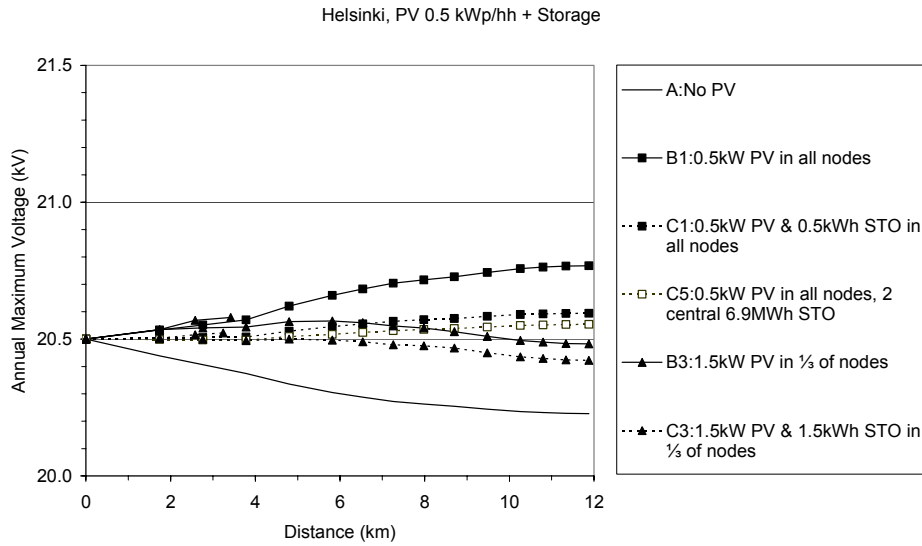
Figure 4.2: Annual maximum voltage profiles in Helsinki for cases A, B1, B3, C1, C3, and C5. The installed PV capacity totals 0.5 \text{ kW}_p / \text{hh} and the corresponding storage capacity 0.5 \text{ kWh} / \text{hh}
