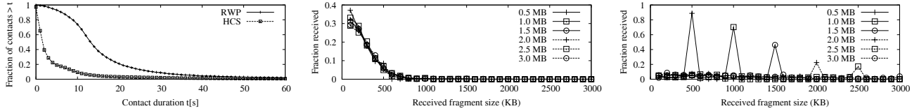
Figure 4. Contact duration (left); received fragment size distribution: HCS (center) and RWP (right)
