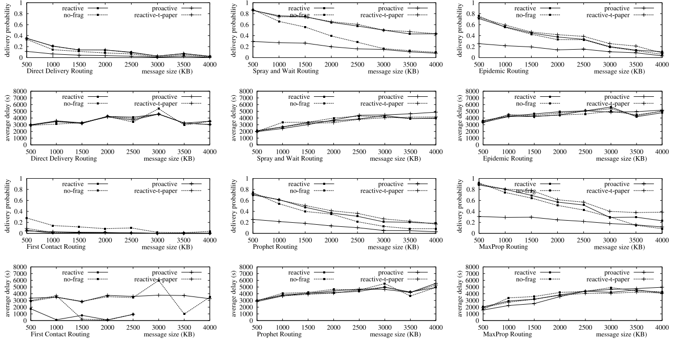
Figure 2. HCS mobility. Delivery probabilities (1st and 3rd row) and latencies (2nd and 4th row).
