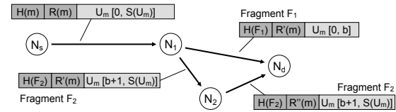
Figure 1. Message fragmentation example
