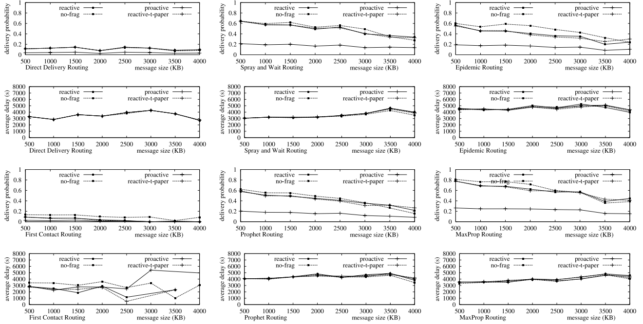
Figure 3. RWP mobility. Delivery probabilities (1st and 3rd row) and latencies (2nd and 4th row).
