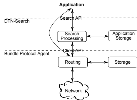
Fig. 6. Components of the DTN-Search Implementation
