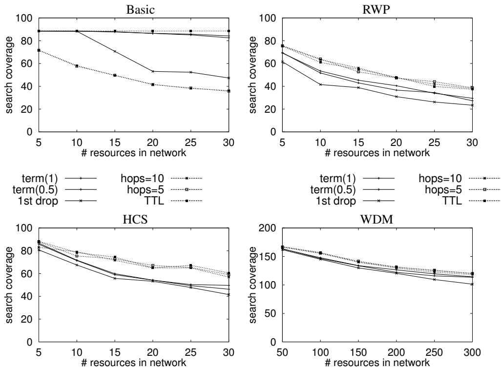
Fig. 4. Search coverage with Epidemic routing.
