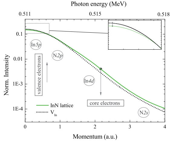
FIG. 2. (Color online) Calculated momentum density of annihilating e - p pairs in the delocalized state of the InN lattice and trapped at the V_{In} , respectively. Trends in the spectra are indicated with respect to the InN lattice.
