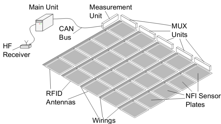
Fig. 24 The pilot system that was built
