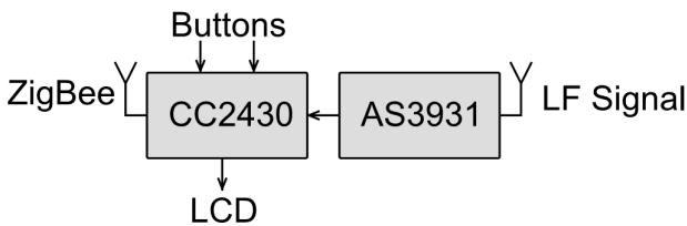
Fig. 23 The tag that was designed and its functional blocks 12
