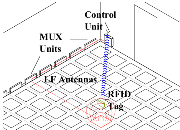
Fig. 14 Dual-signal localization with loop antenna matrix 8
